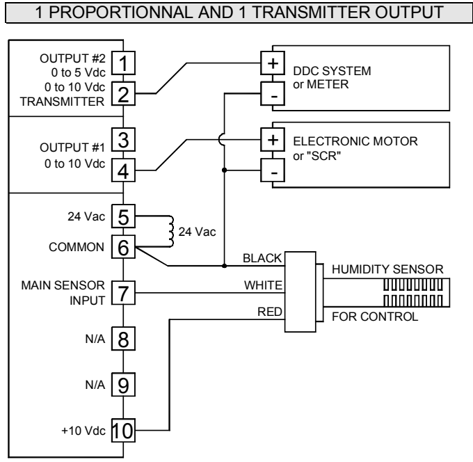
Fig. 5: Wiring diagram with one analog and one transmitter output
